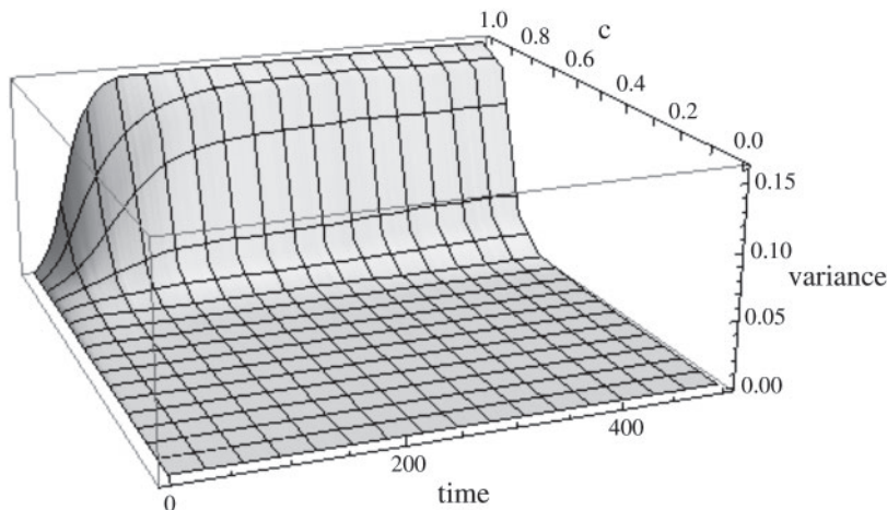
FIG. 2. Variances of cluster sizes for varying values of c . Variances are average values obtained by running 100 simulations for each value of c ( c = 0.0, c = 0.1, \dots, c = 1.0 ). At t = 0 all clusters start with the same size, hence variance is 0. All simulations were run with 500 agents, 5 clusters, and 500 periods.
